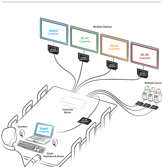
Secure Isolator System Diagram
